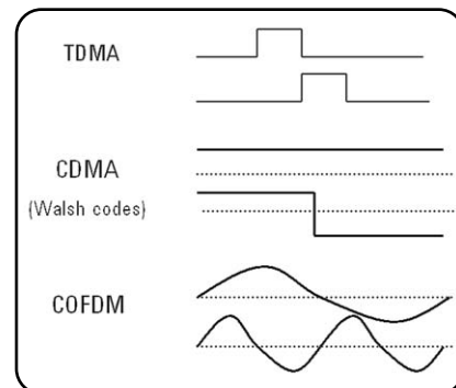
Figure 3.1.1. Orthogonal signals
