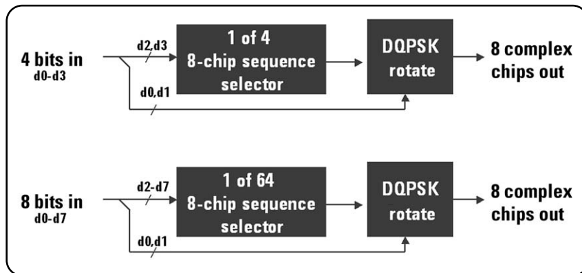
Figure 2.2.1. CCK modulation
