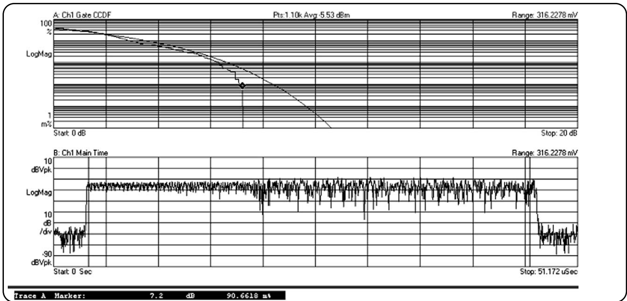
Figure 3.3.9. CCDF curve
